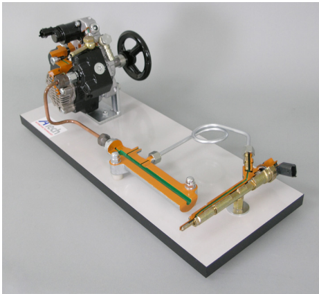
Common Rail Diesel Cutaway Model 10300
