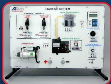
Starting System (811C)
