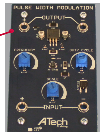
Pulse Width Modulation 500-009-001
