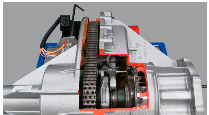
Transfer Case (High Range Position) (Model 1230)
