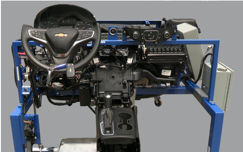
Engine Performance Trainer Model 650
