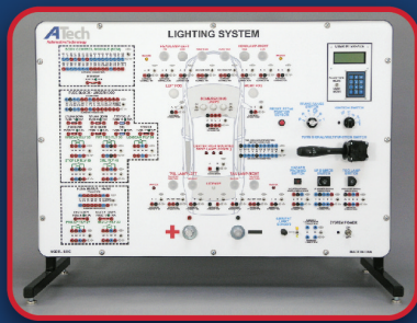
Lighting System (821C)
